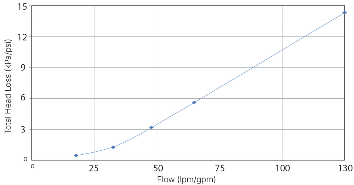
Head Loss
